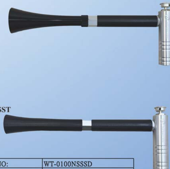
WT-0100NSS Palm-grip Blow Gun (Ø32mm Nozzle) Schematic Diagram of Installing the Extension Rod
